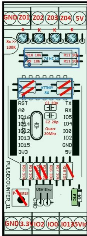
Platine pulsecounter_11
